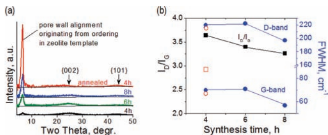
Figure 2. Microstructure of zeolite Y-templated carbons synthesized at 700 °C for 4, 6 and 8h: (a) XRD and (b) Raman analyses. The background in panel a was removed. Values in panel b for the annealed sample are shown by unfilled symbols.
