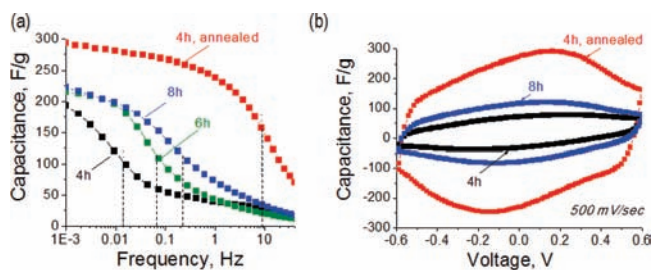
Figure 3. Effect of pore alignment in zeolite Y-templated carbons on ion transport in EDLC: (a) estimated capacitance retention with increasing operating frequency, (b) cyclic voltammetry recorded at ultrafast sweep rate of 500 mV/s; 1 M H 2 SO 4 was selected as electrolyte.
