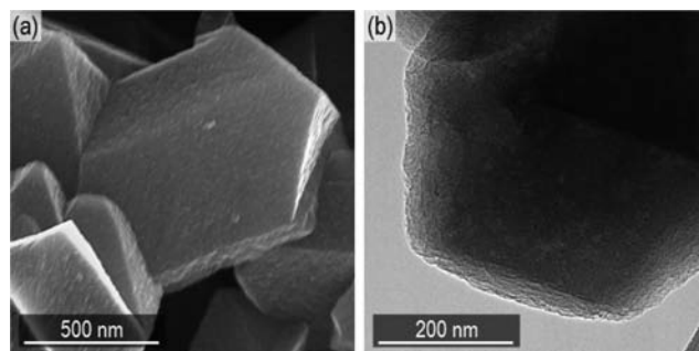
Figure 1. Electron microscopy of zeolite Y-templated carbons: (a) scanning and (b) transmission electron microscopy (SEM and TEM) images of synthesized porous carbon particles produced at 700 °C.
